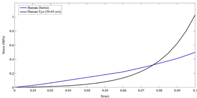
Figure 3: Tensile stress-strain curve for decellularized dermis obtained from tensile stress-strain measurements and human eyes from inflation tests. Note the similarity between the shapes of the stress-strain curve for decellularized dermis composed largely of type I collagen and that of whole eyes. The upward curvature involves increased recruitment of collagen fibers with the loading direction with increasing strain and leads to the increased slope of the stress-strain curve.
