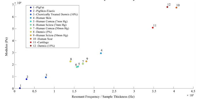
Figure 5: Plot of vibrational modulus versus the ratio of the resonant frequency per unit thickness for human decellularized dermis, human skin and scar, bovine cartilage, porcine fat and human cornea and sclera. The modulus for fat is about 0.03 MPa, elastic tissue 0.4 to 0.8 MPa, and collagen 2.0 to 7.0 MPa. Normal skin has a modulus of about 2 MPa and scar of about 7 MPa. Normal cornea and sclera have moduli of about 2 MPa at low and high intraocular pressures very similar to normal skin. Note that softening or stiffening of the ECMs found in ocular tissues would lead to lower (chemically treated dermis) or higher (scar) values of the moduli, respectively that would be measureable using vibrational OCT.
