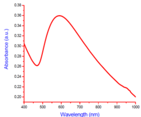
Figure 2: UV-Visible spectrum of 0.5 wt% Cu nanoparticles-PVP suspension.
