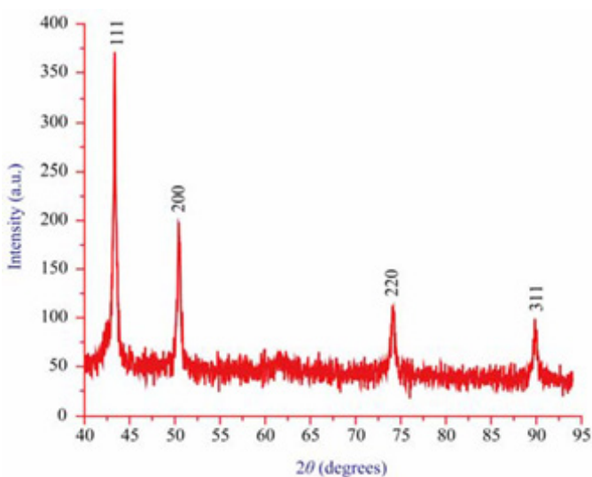
Figure 6: XRD pattern of 0.5 wt% Cu nanoparticles-PVP suspension.
