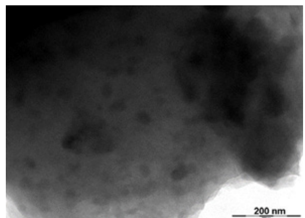
Figure 3: TEM micrograph of 0.2 wt% Cu nanoparticles-PVP suspension.
