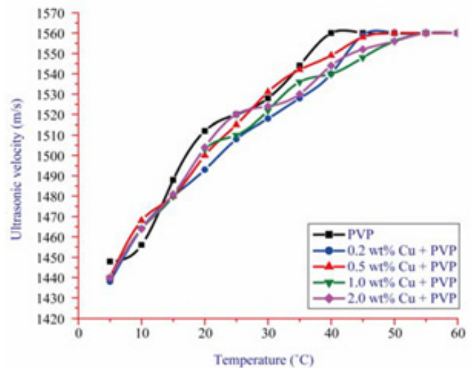
Figure 8: Temperature dependent ultrasonic velocity in Cu-PVP nanofluids.
