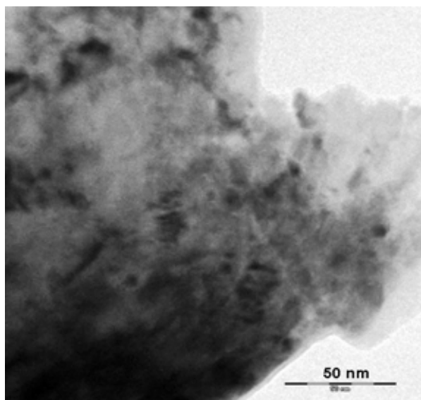
Figure 5: TEM micrograph of 2.0 wt% Cu nanoparticles-PVP suspension.
