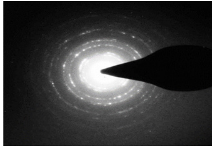
Figure 7: SAED pattern of 0.5 wt% Cu nanoparticles-PVP suspension.
