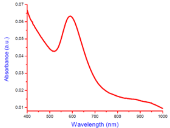
Figure 1: UV-Visible spectrum of 0.2 wt% Cu nanoparticles-PVP suspension.
