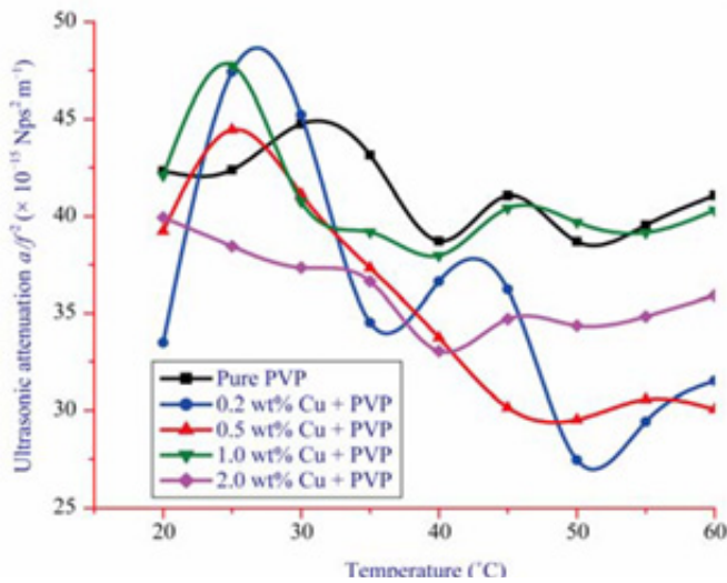
Figure 9: Temperature dependent ultrasonic attenuation in Cu-PVP nanofluids.
