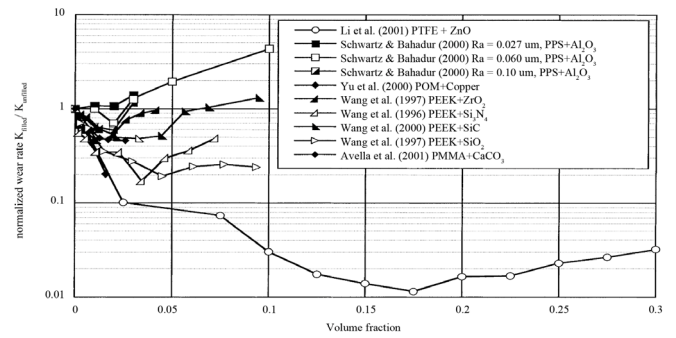
Figure 1: A plot of normalized wear improvements for polymer nano-composites as a function of filler volume fraction.
